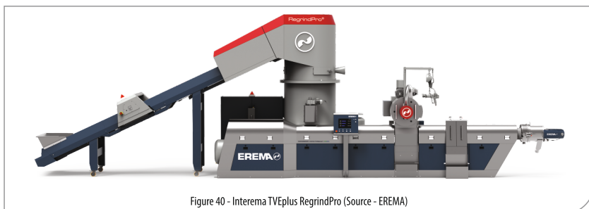
Figure 40 - Intarema TVEplus RegrindPro (Source - EREMA)
