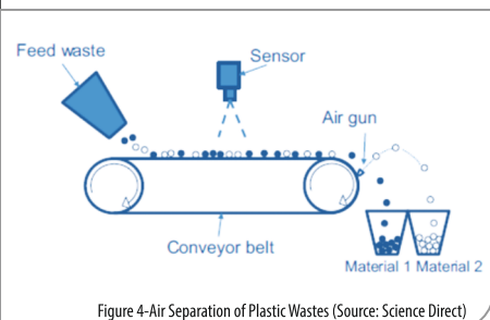
Figure 4-Air Separation of Plastic Wastes (Source: Science Direct)
